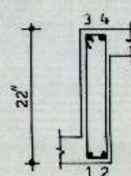
BEAM B-2
