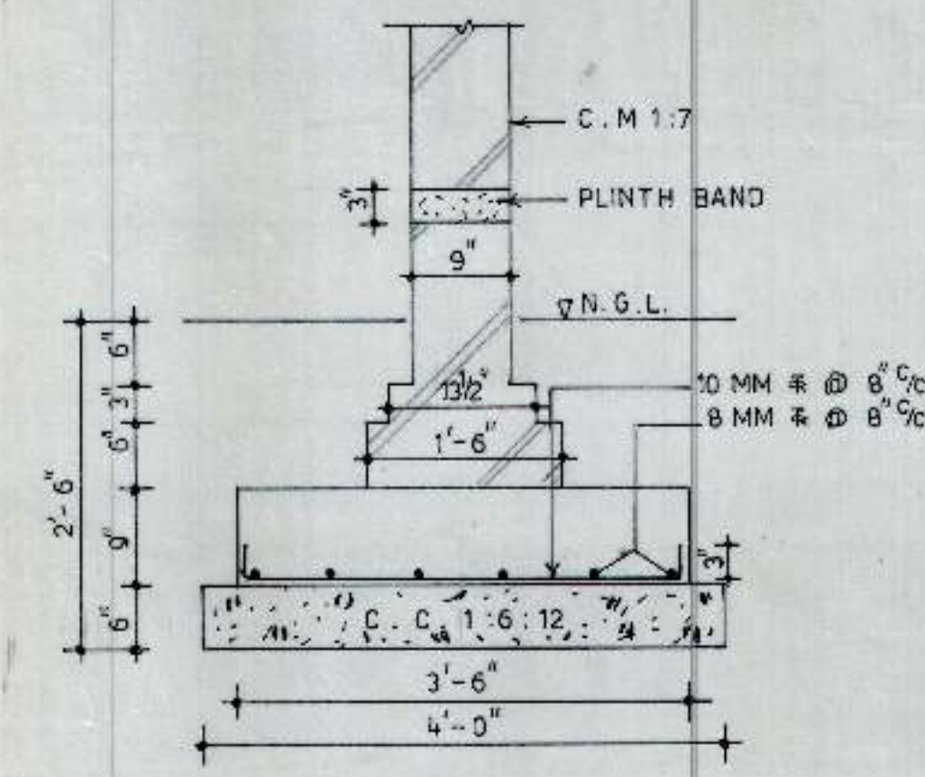
WALL W-4
