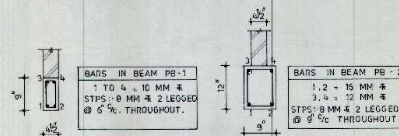
BEAM PB-1
