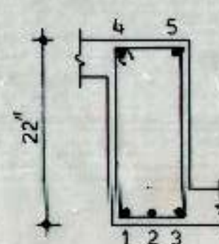
BEAM B-1
