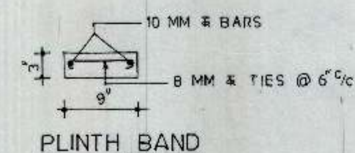
BEAM PB-1
