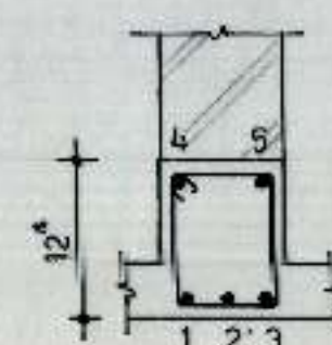
BEAM B-3
