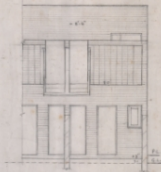
SECTIONAL ELEVATION C-C
