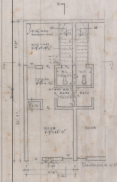
PHASE II GROUND FLOOR PLAN
