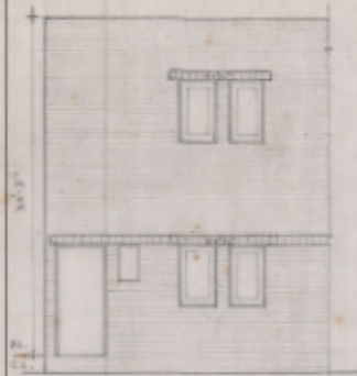
FRONT ELEVATION
