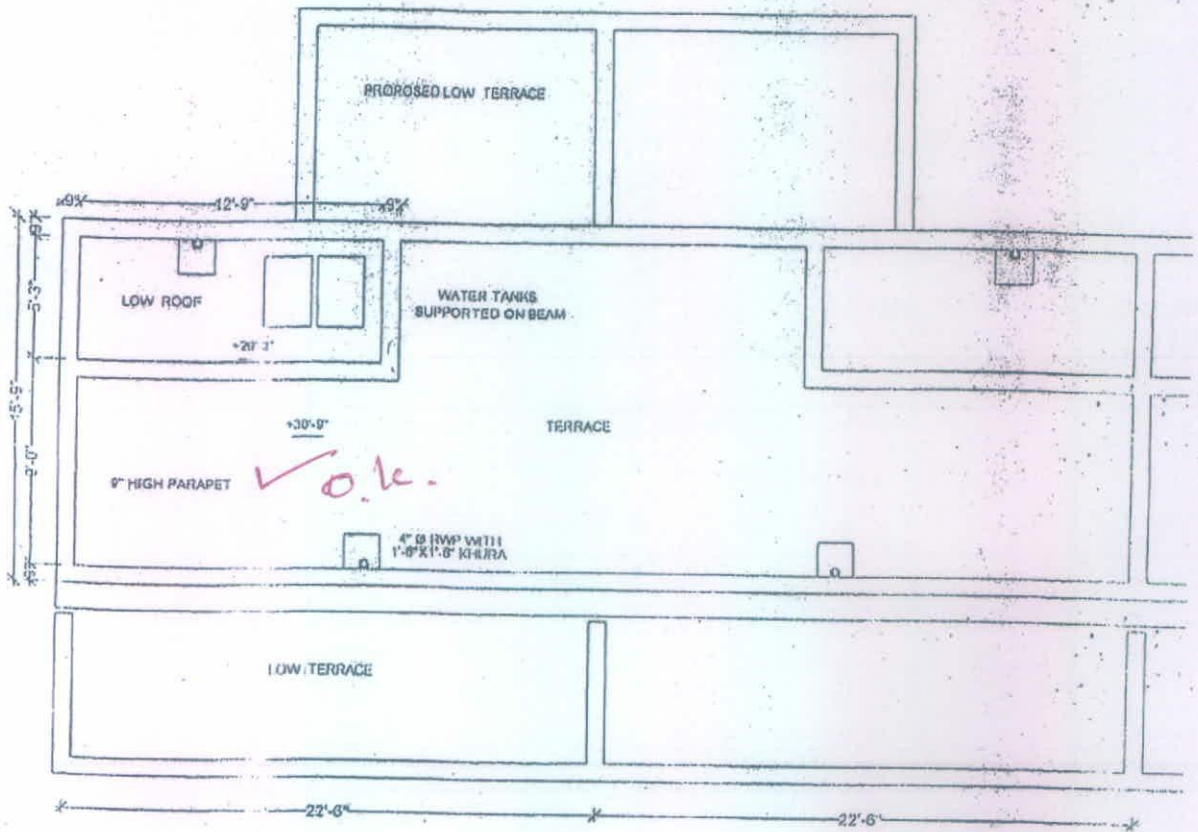
TERRACE PLAN
