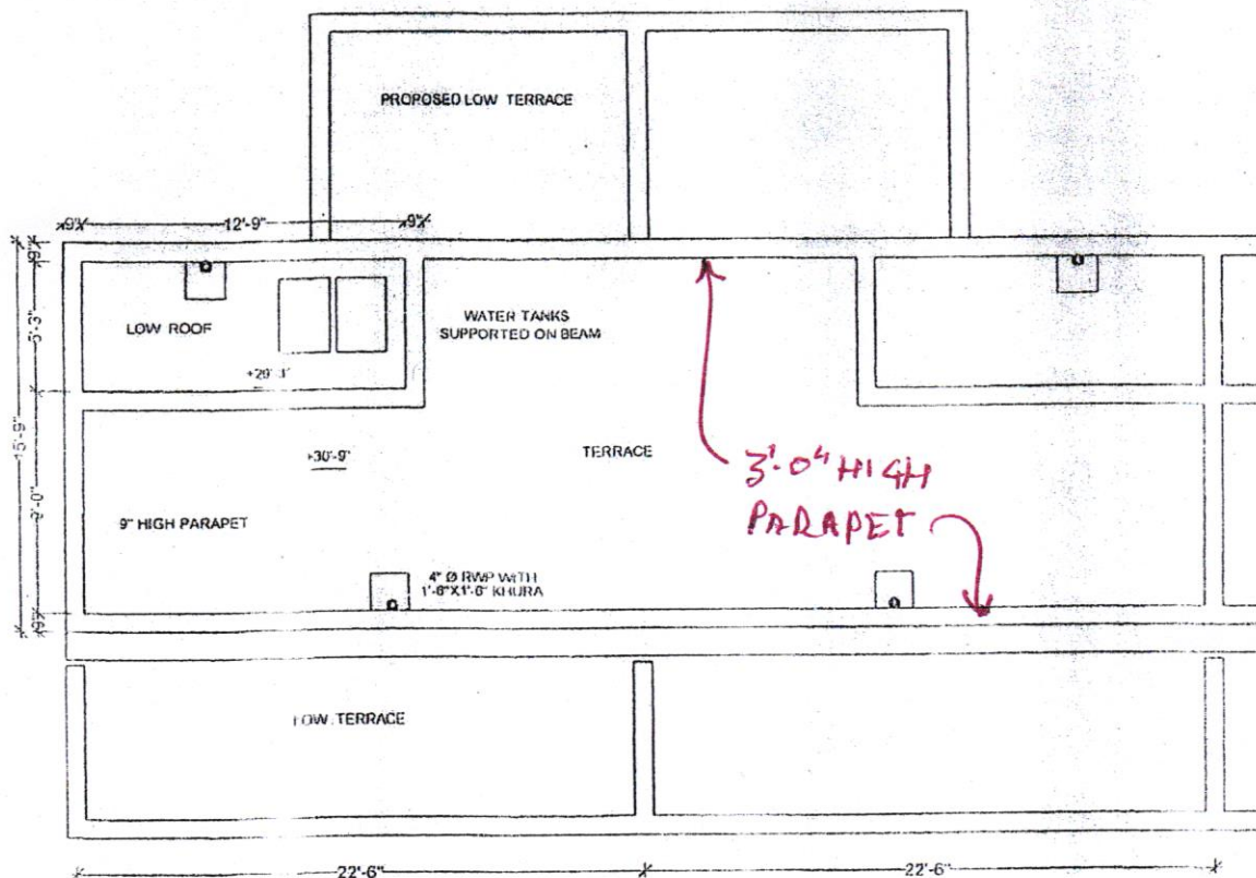
TERRACE PLAN
