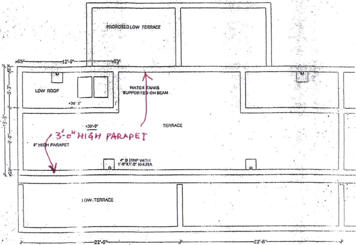
TERRACE PLAN
