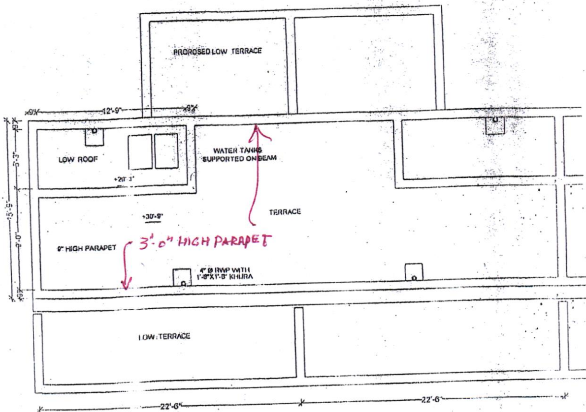
TERRACE PLAN
