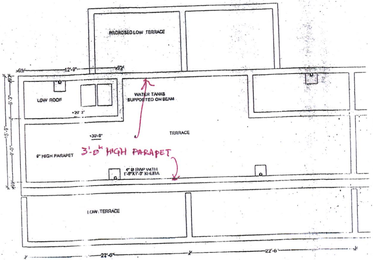
TERRACE PLAN
