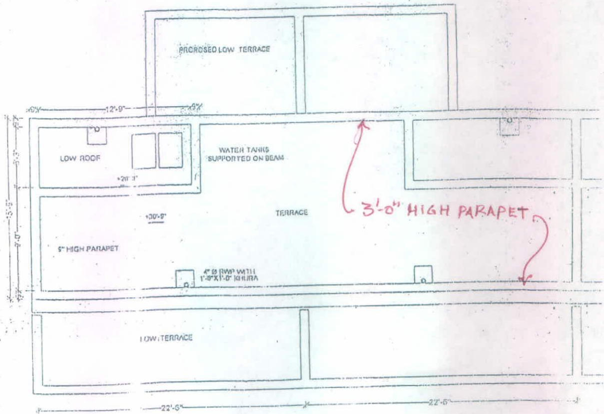
TERRACE PLAN
