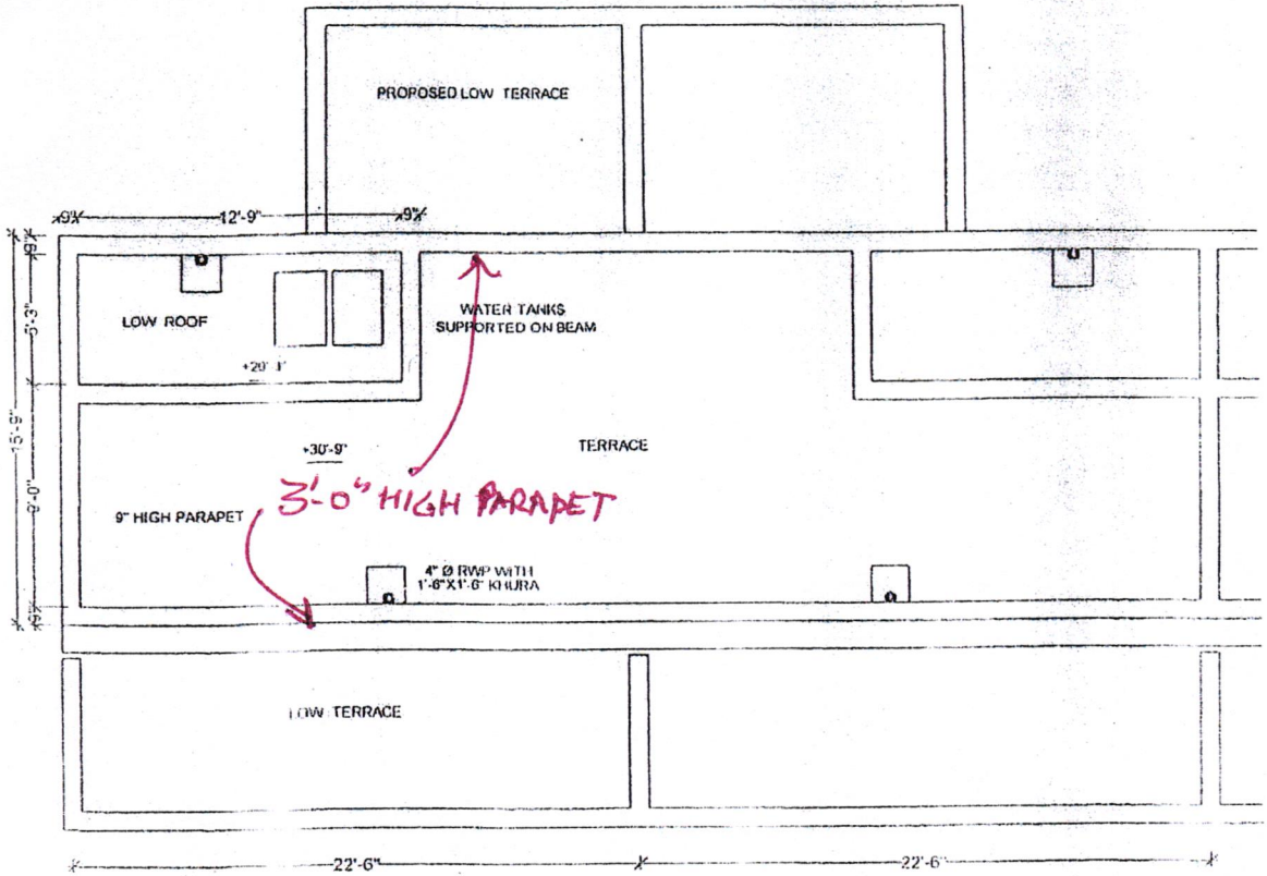
TERRACE PLAN
