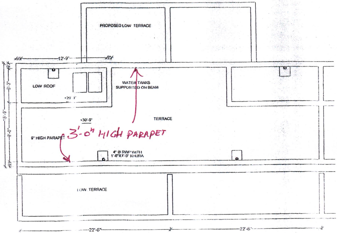
TERRACE PLAN
