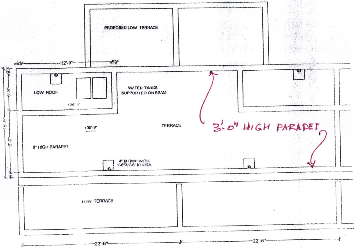
TERRACE PLAN
