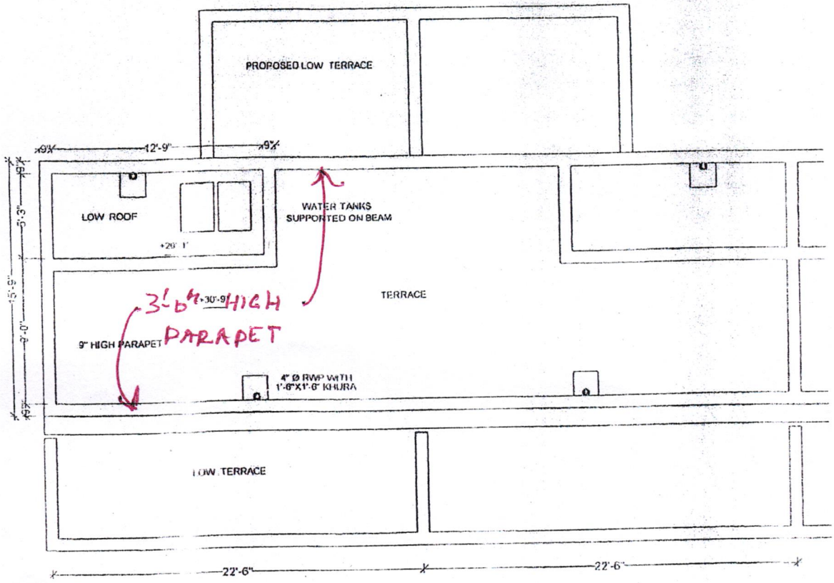
TERRACE PLAN
