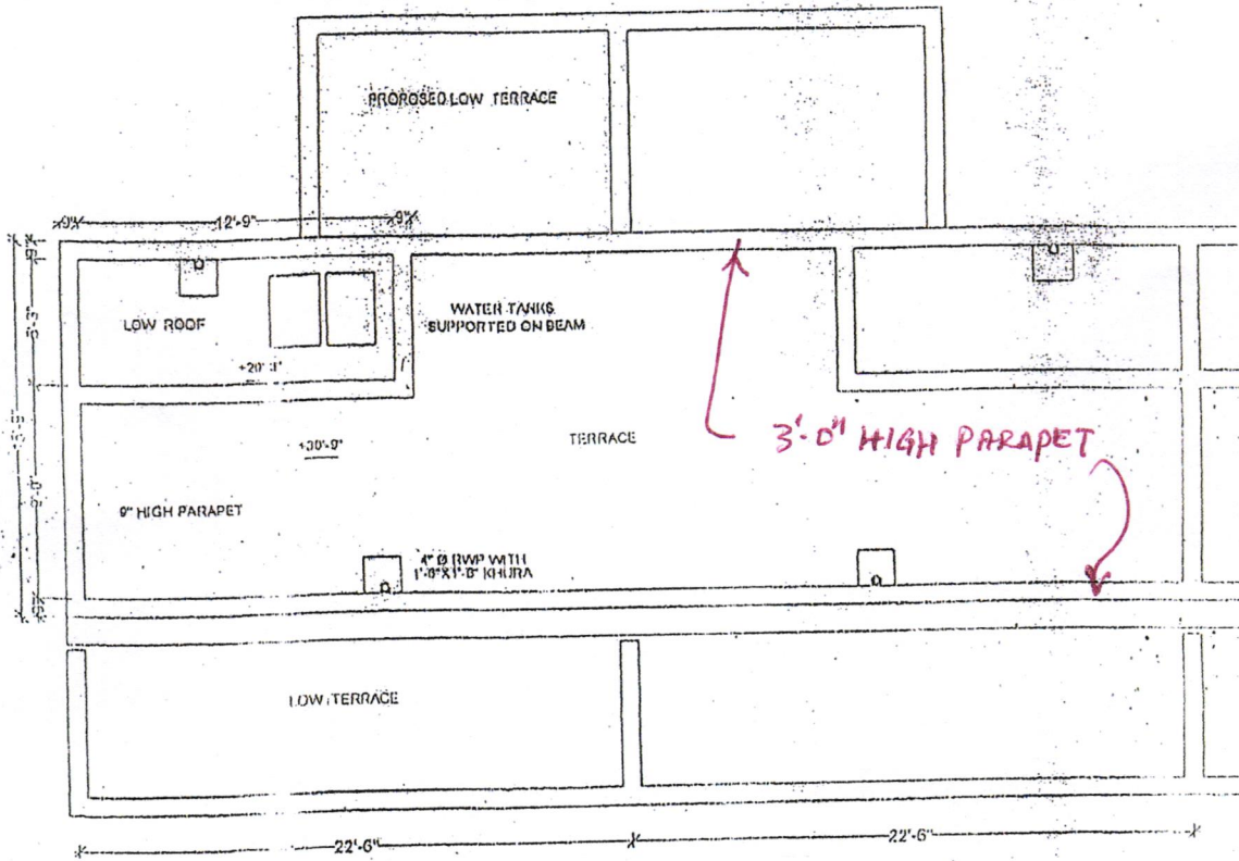
TERRACE PLAN
