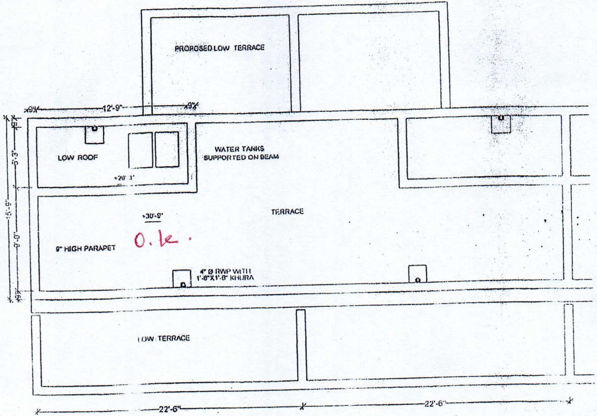
TERRACE PLAN
