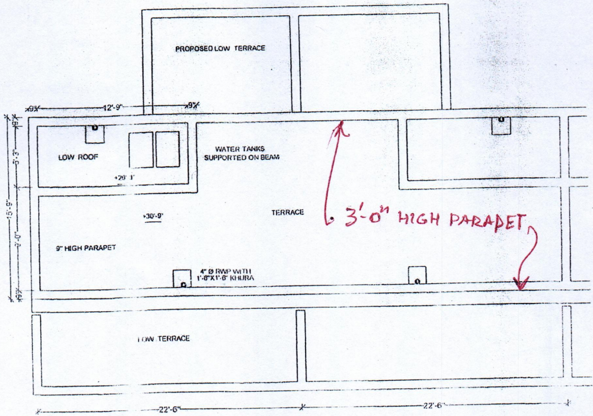
TERRACE PLAN
