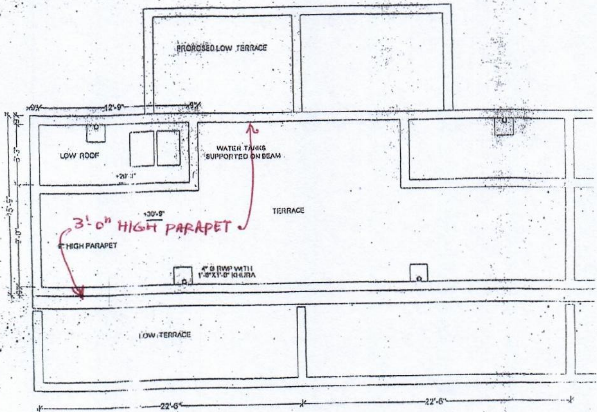
TERRACE PLAN
