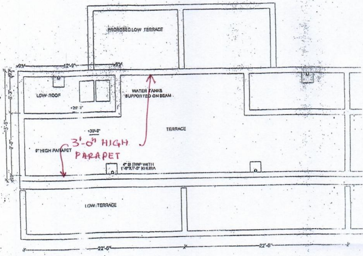
TERRACE PLAN
