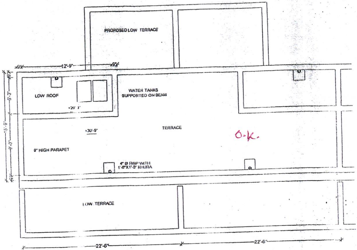
TERRACE PLAN
