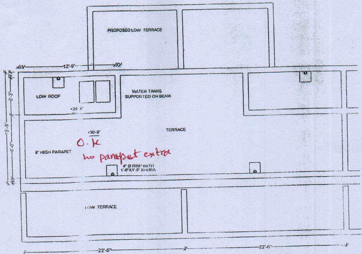
TERRACE PLAN
