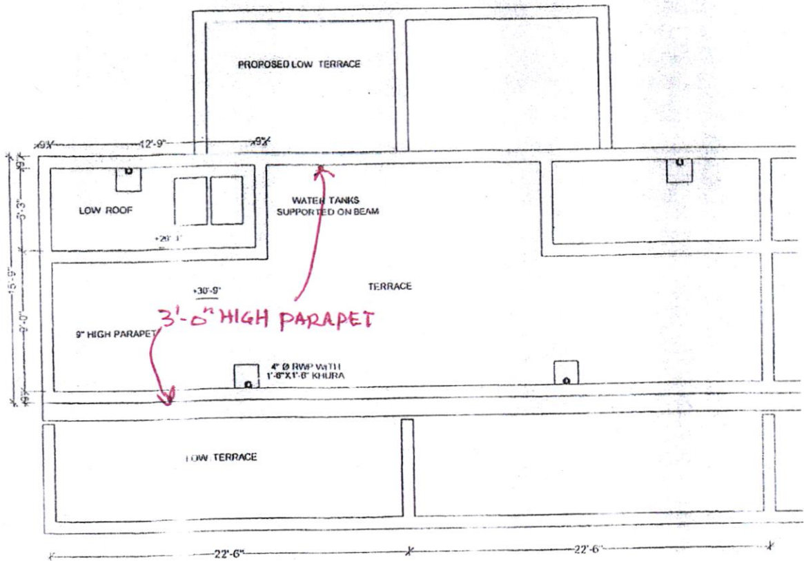
TERRACE PLAN
