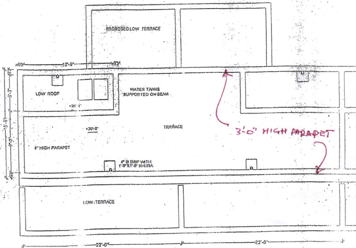
TERRACE PLAN
