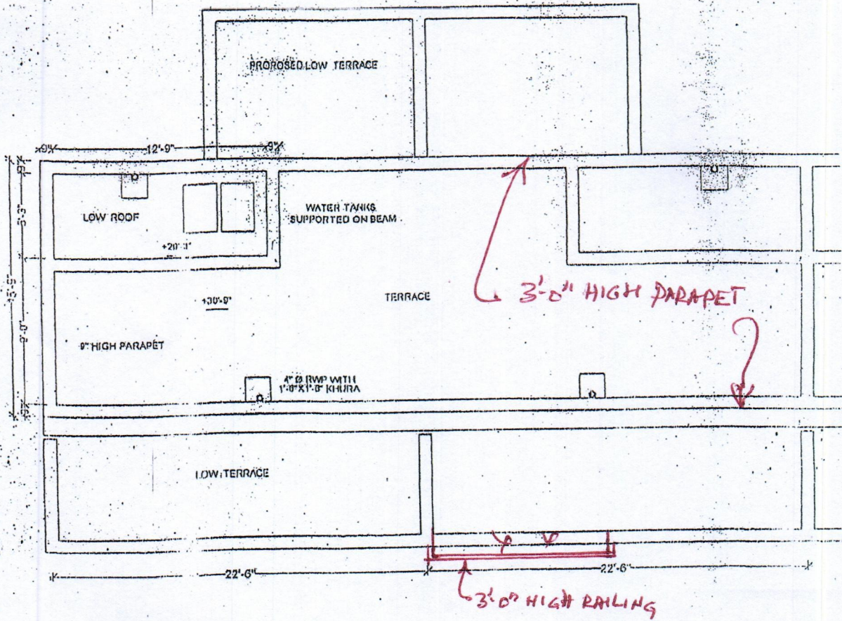
TERRACE PLAN
