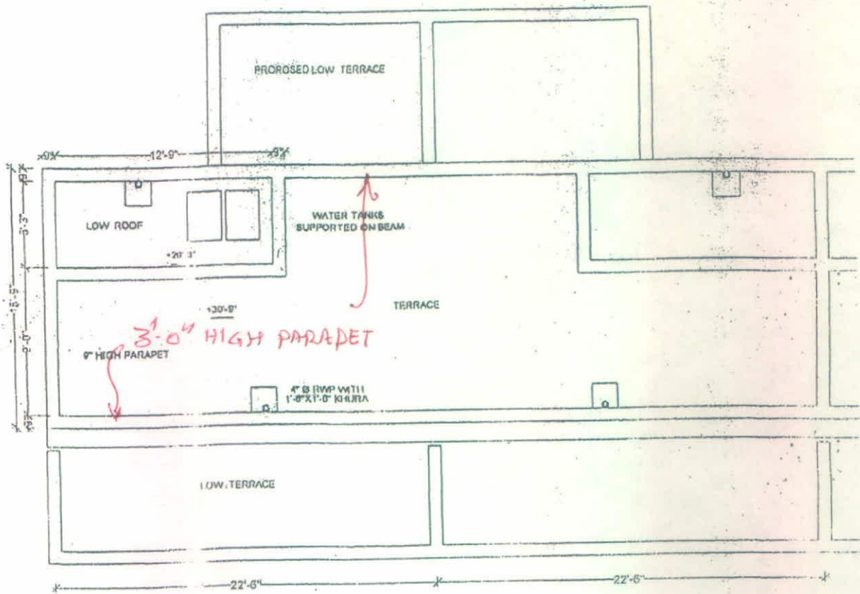
TERRACE PLAN
