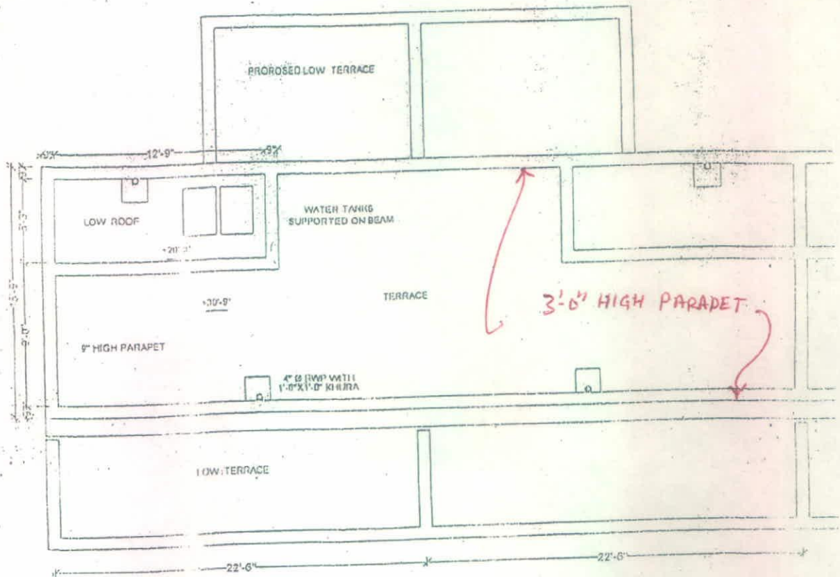
TERRACE PLAN
