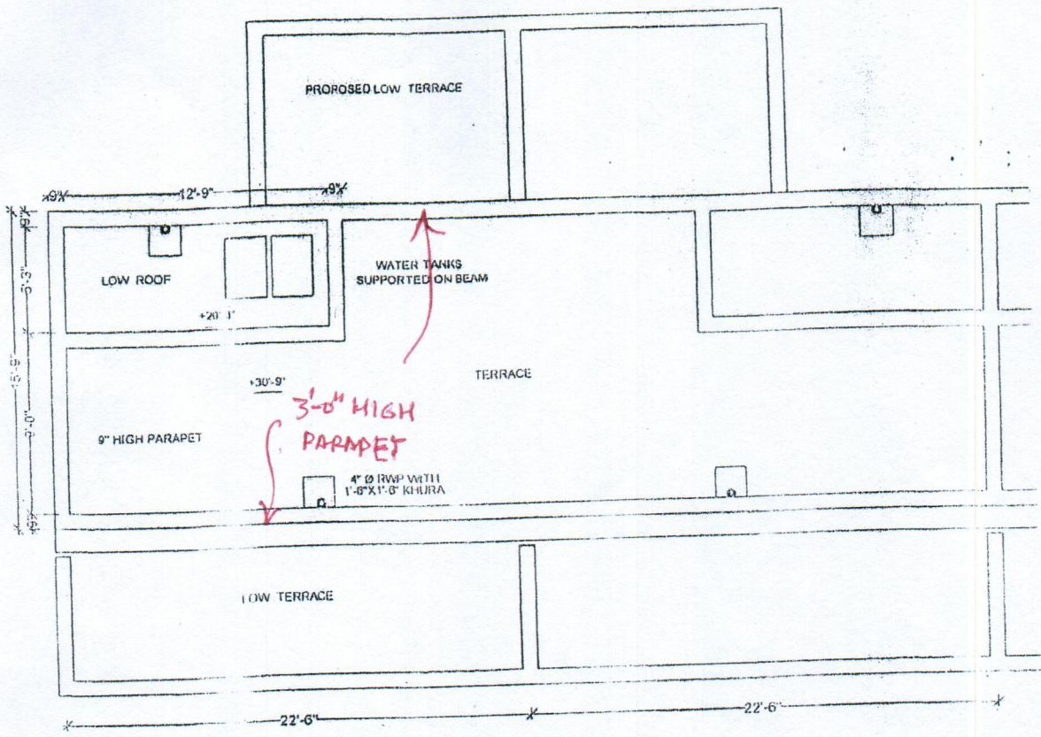
TERRACE PLAN
