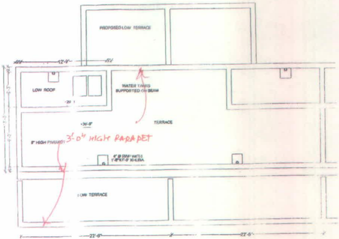
TERRACE PLAN
