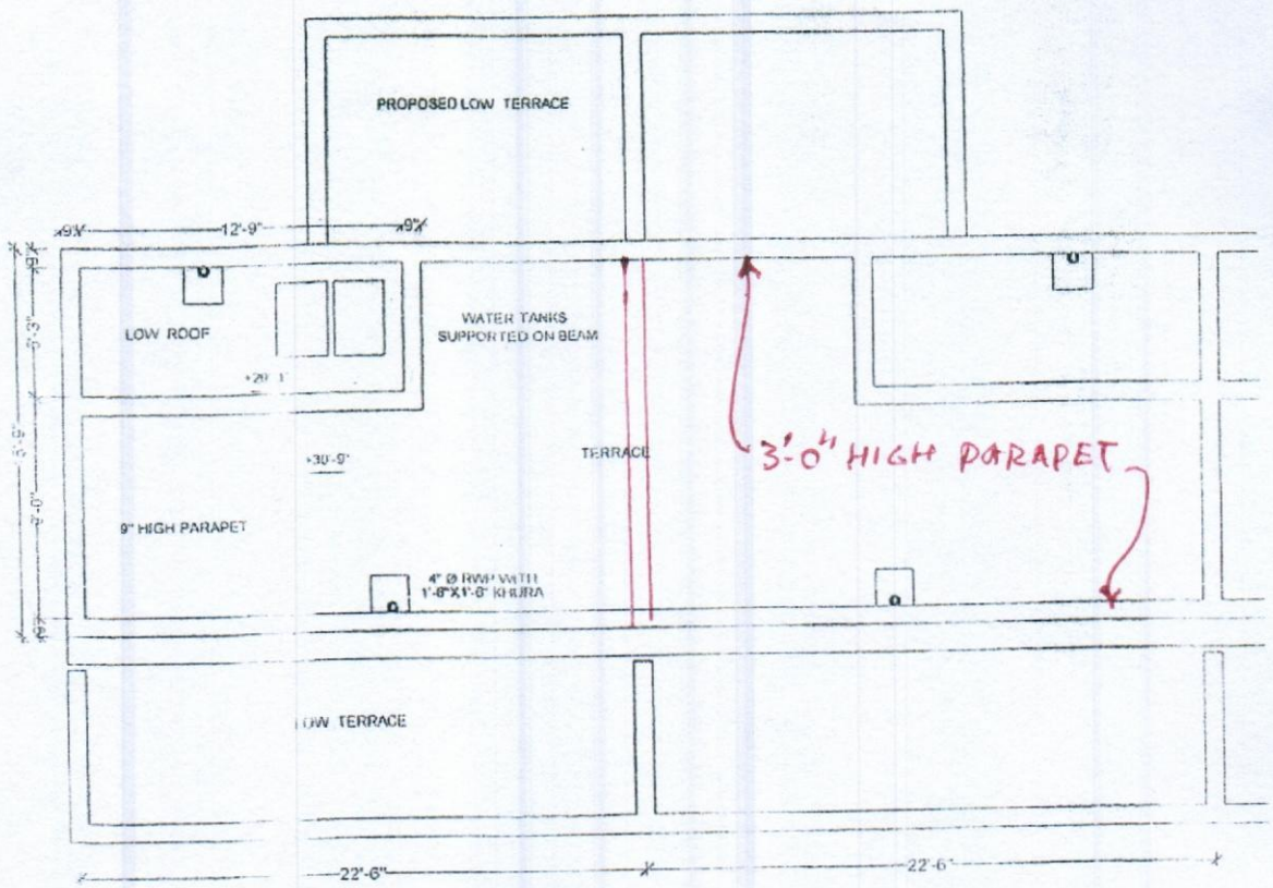
TERRACE PLAN H.No. 756/1
