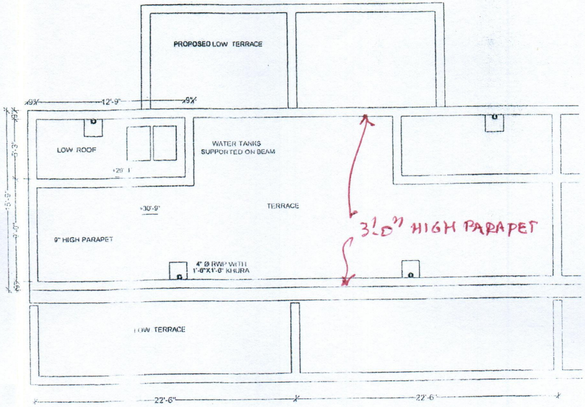
TERRACE PLAN H- No. 762/1
