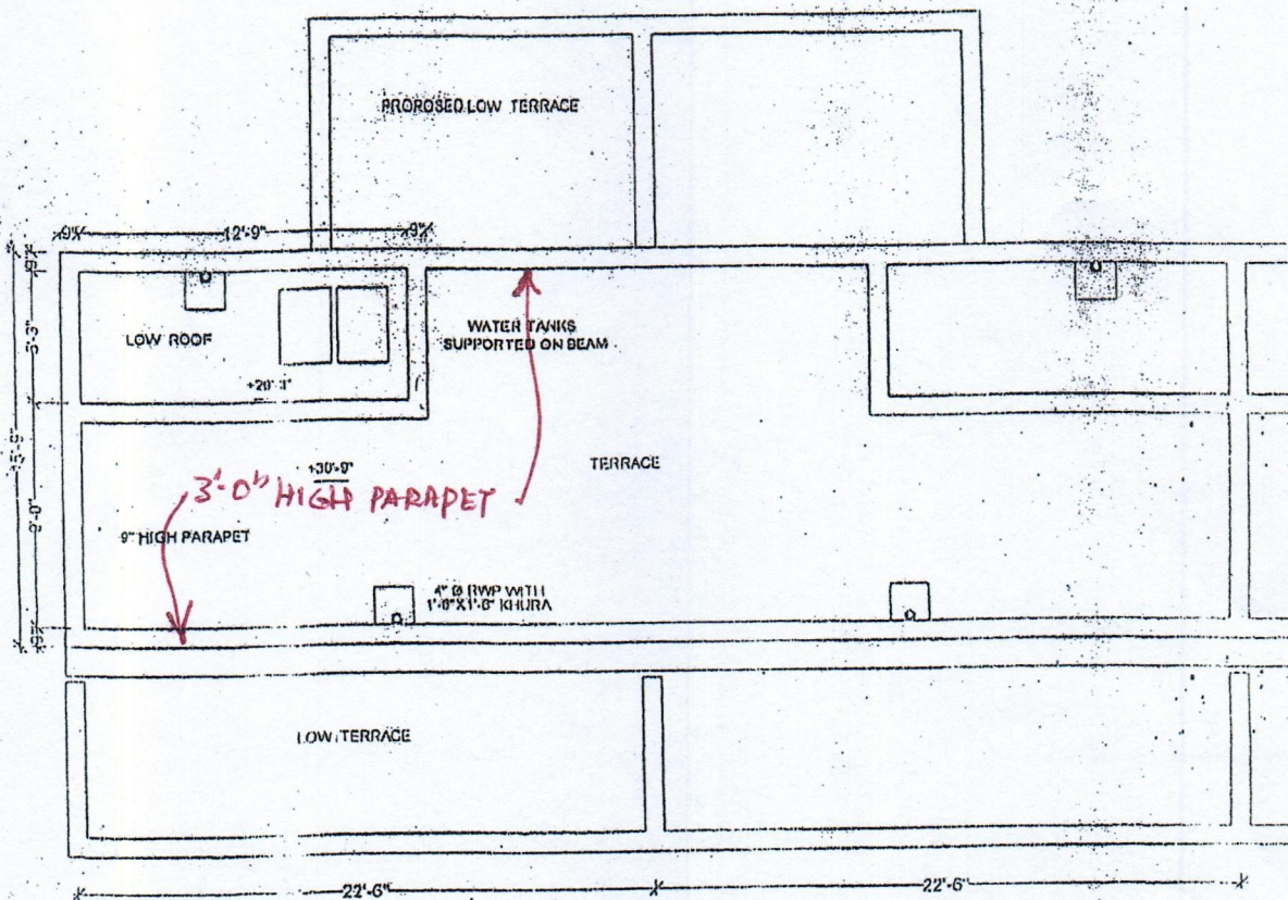
TERRACE PLAN # 767/1, SEC. 41-A
