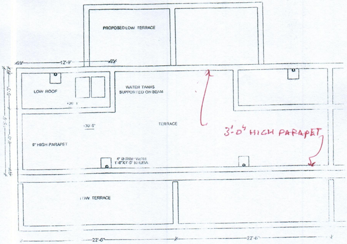
TERRACE PLAN H. No. 778/1
