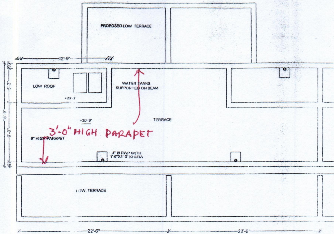
TERRACE PLAN
