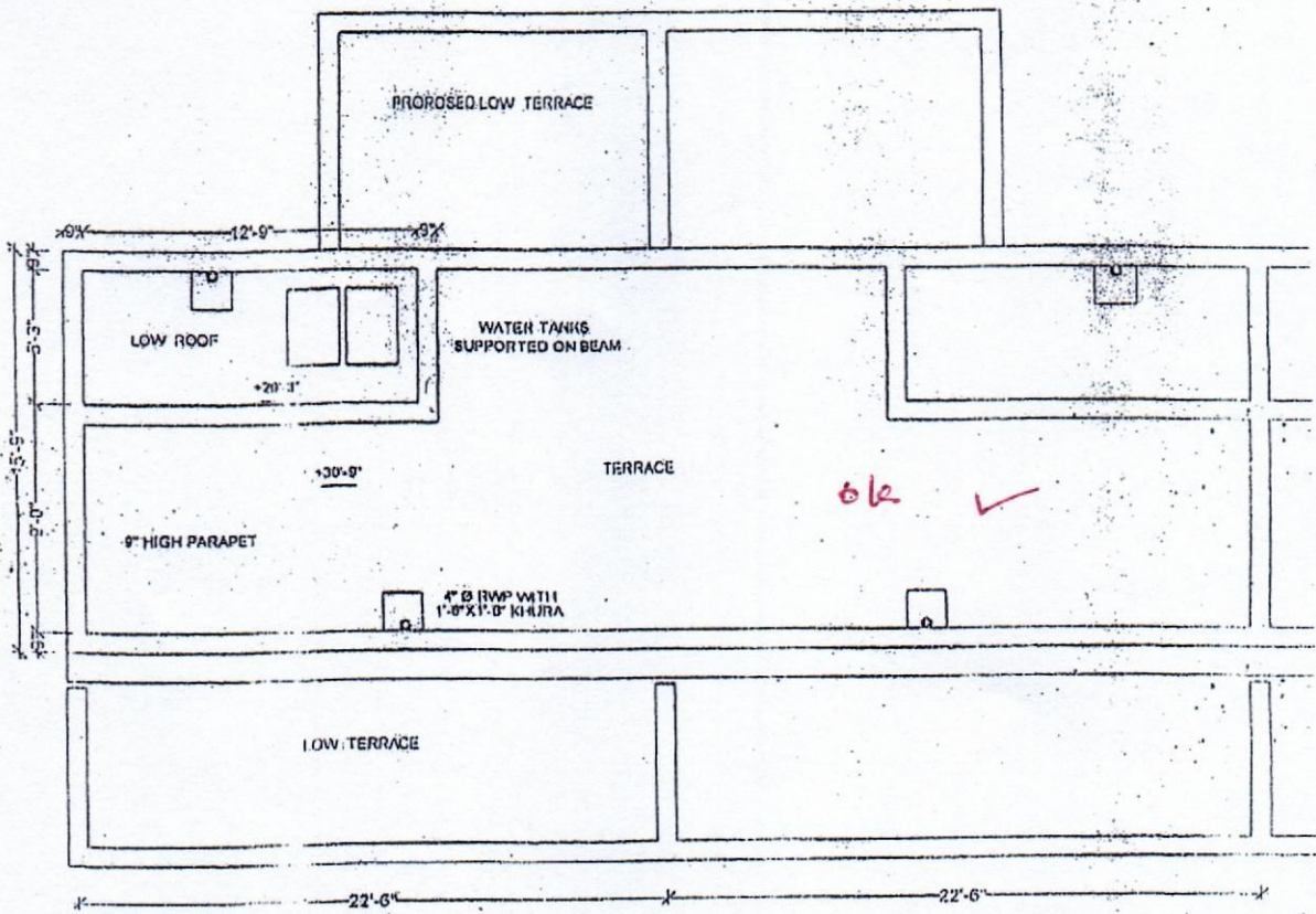
TERRACE PLAN
