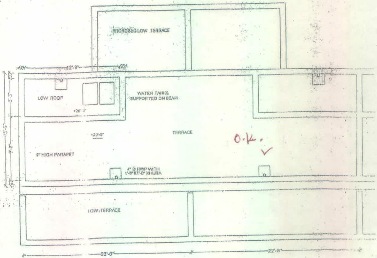
TERRACE PLAN
