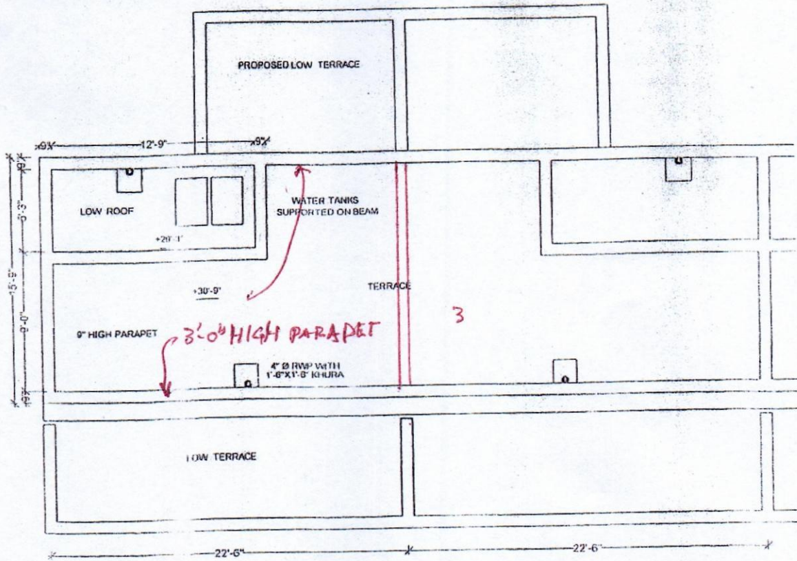
TERRACE PLAN
