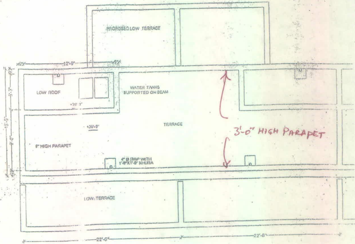
TERRACE PLAN
