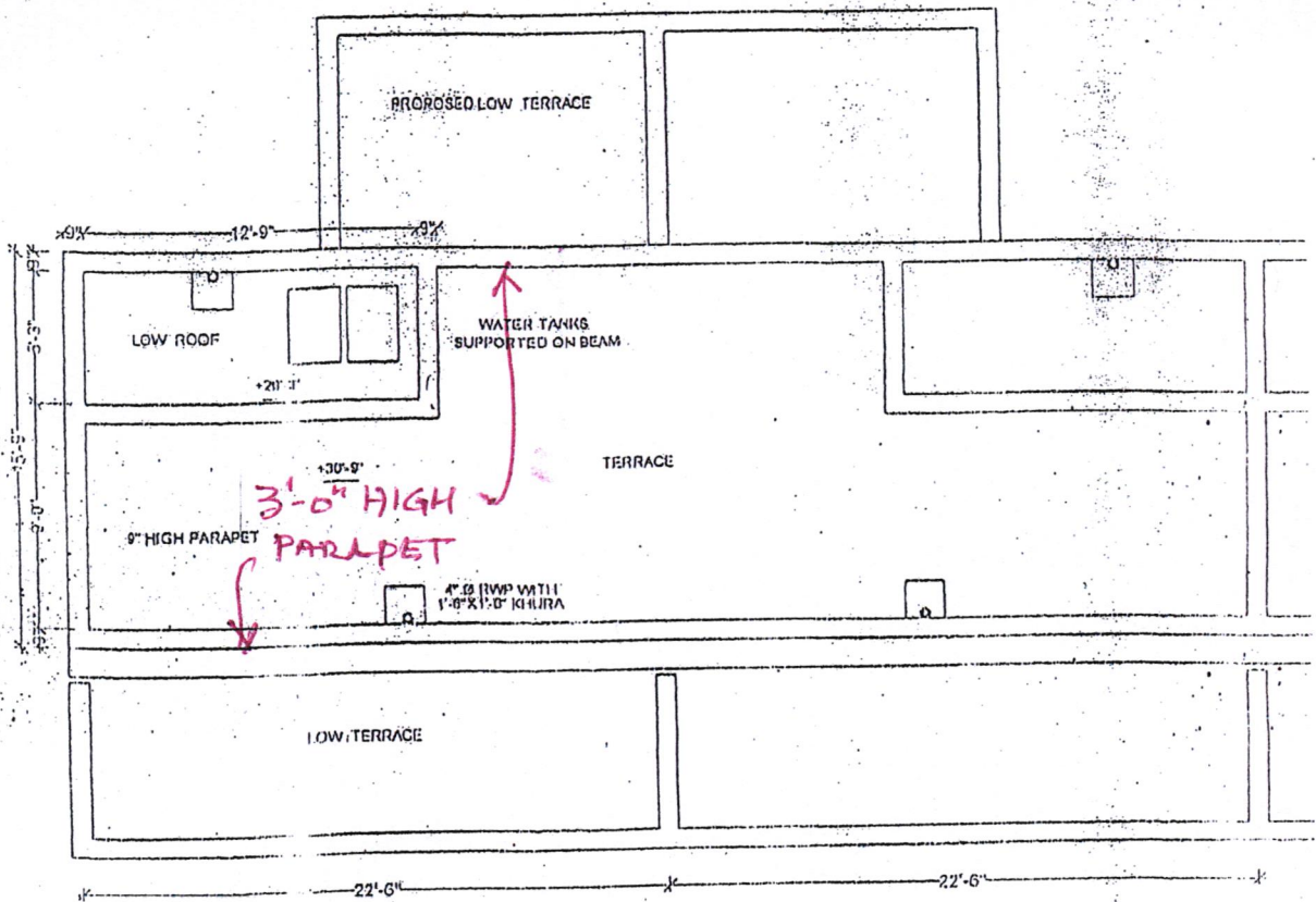
TERRACE PLAN
