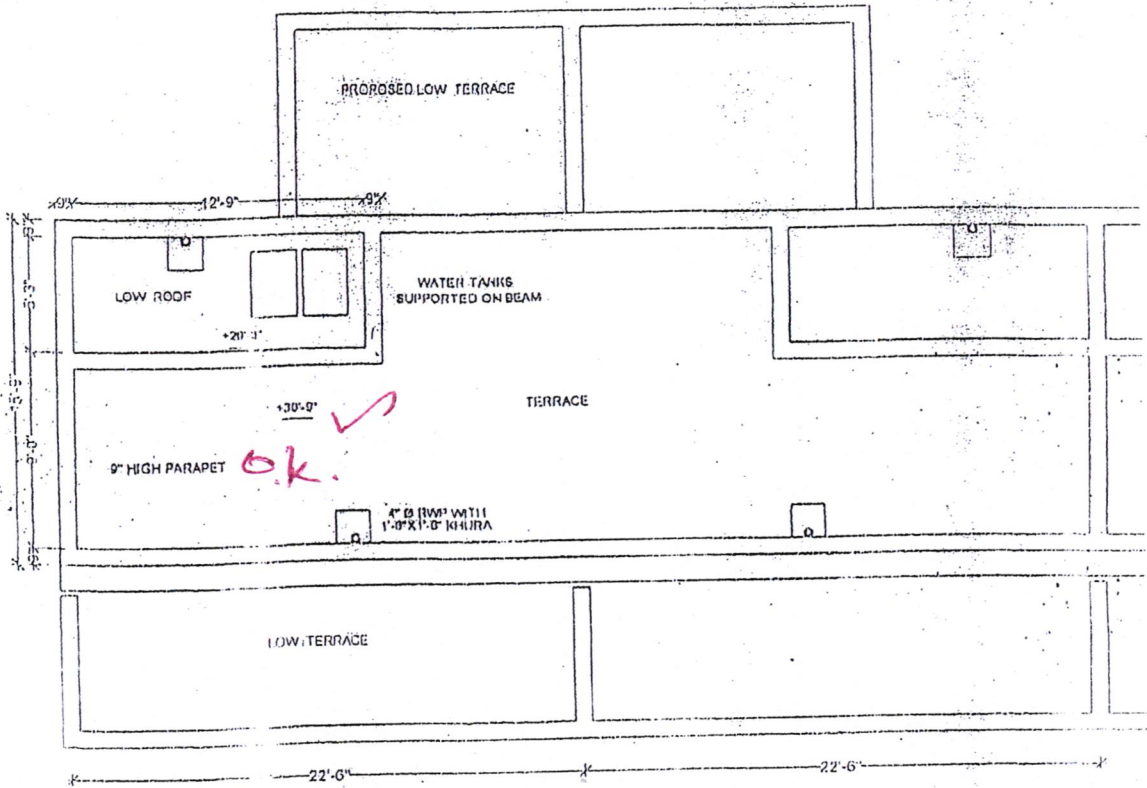
TERRACE PLAN
