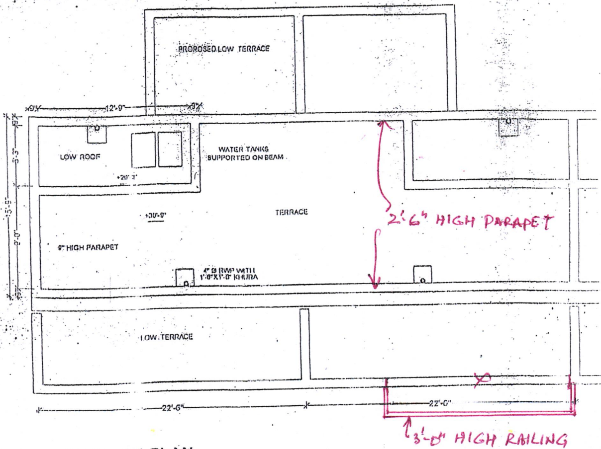
TERRACE PLAN
