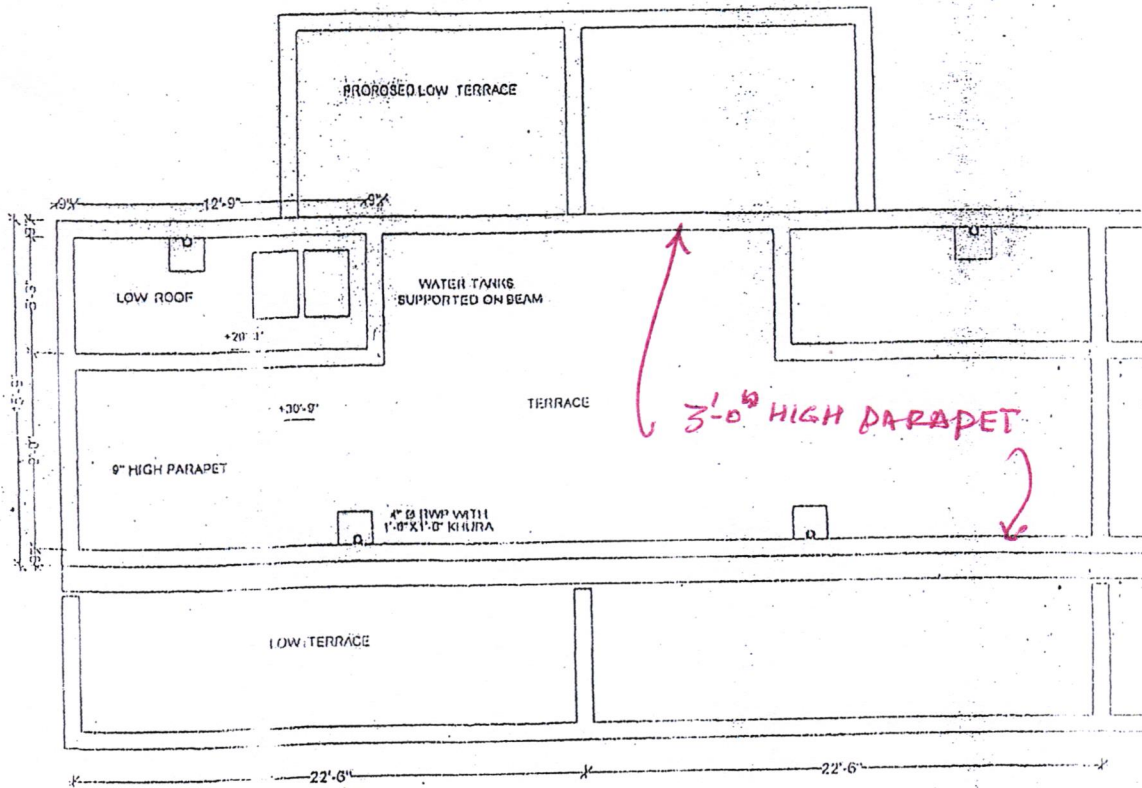
TERRACE PLAN
