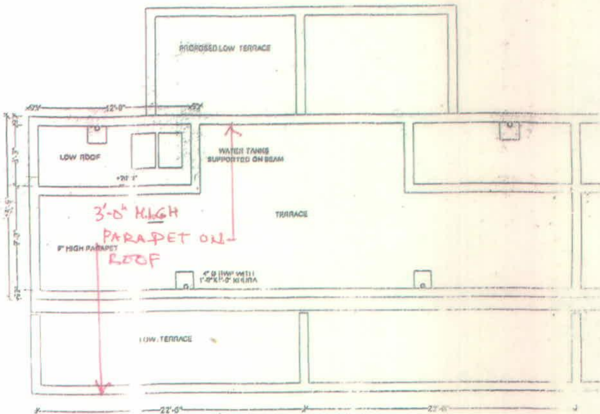
TERRACE PLAN
