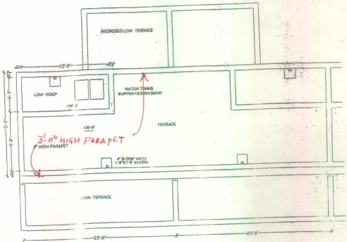
TERRACE PLAN
