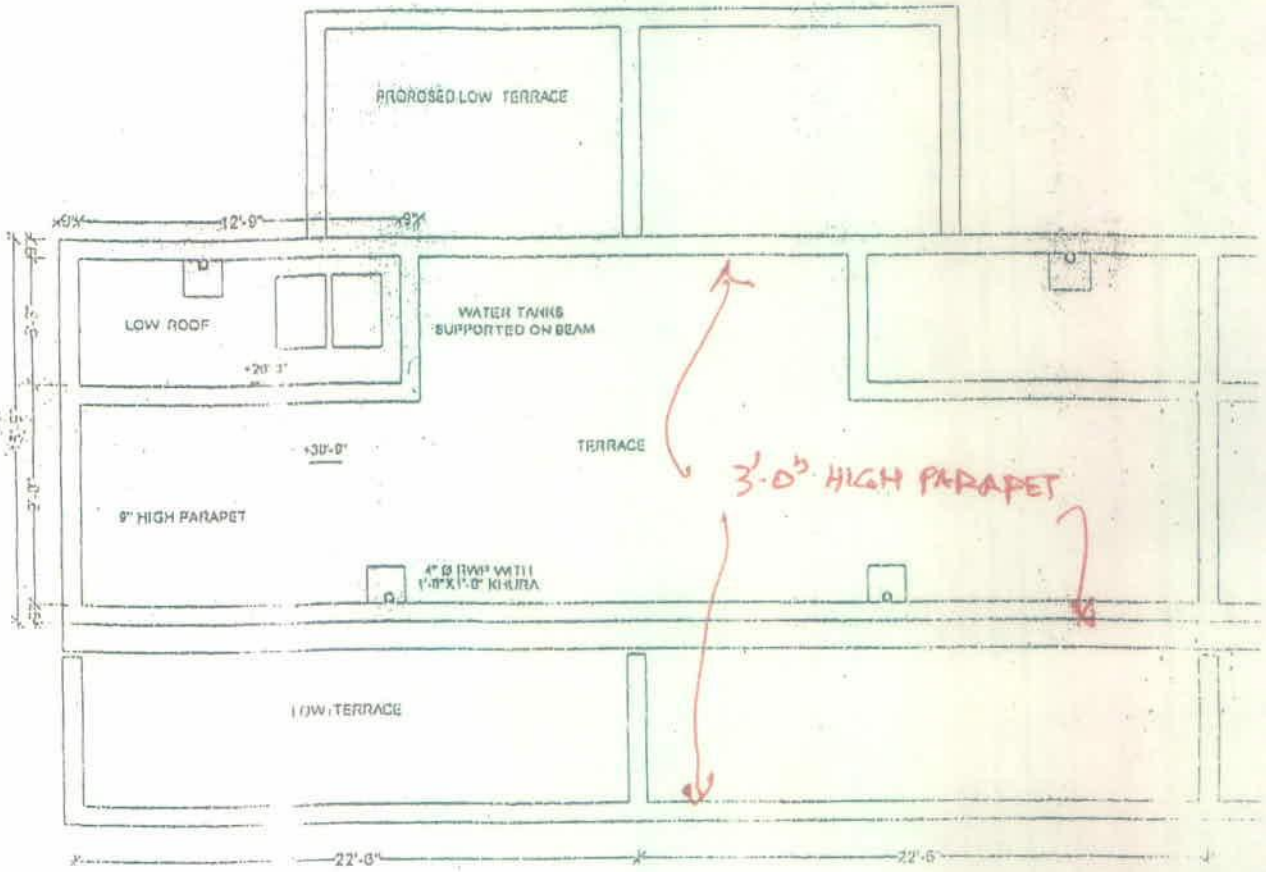
TERRACE PLAN
