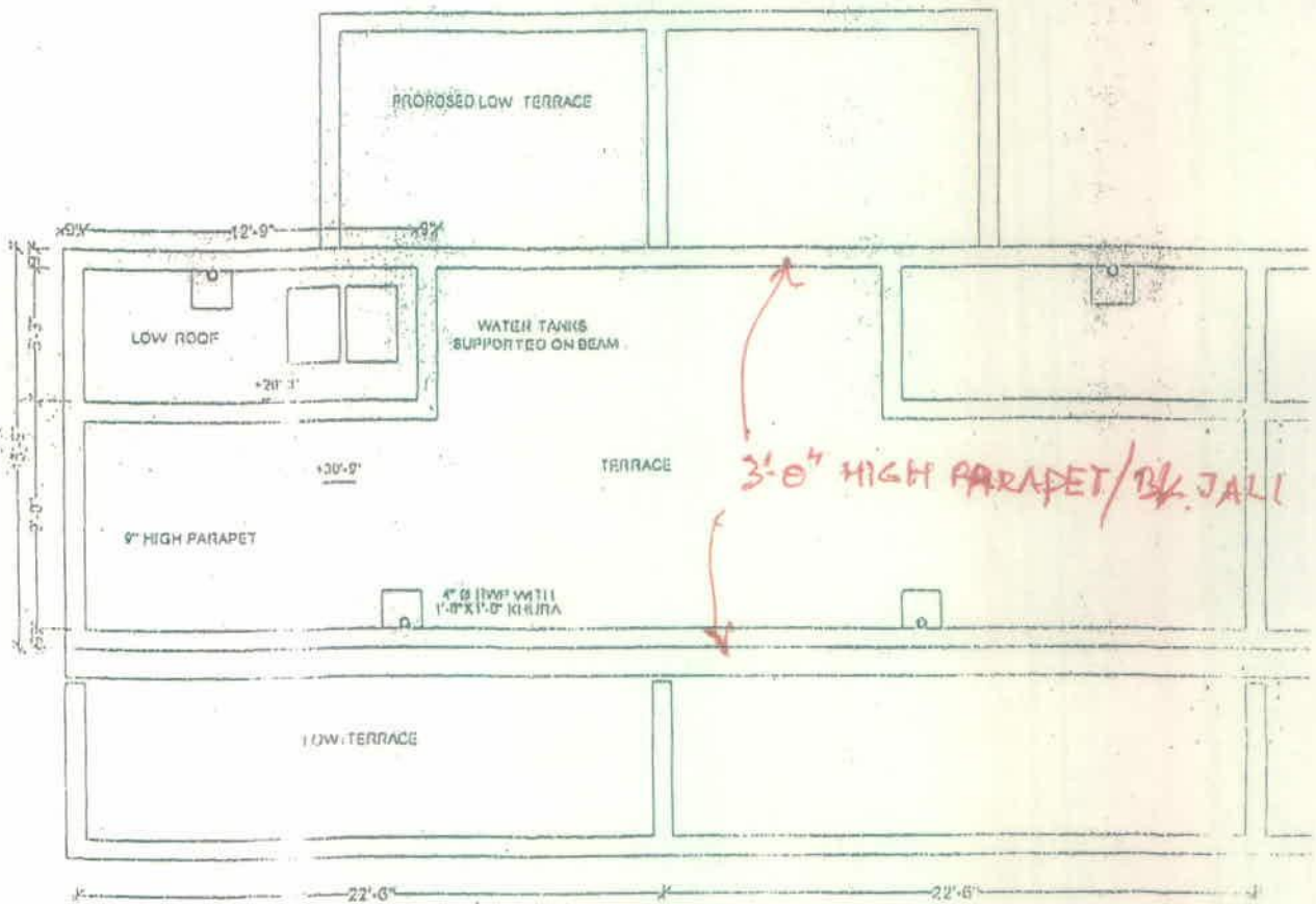
TERRACE PLAN
