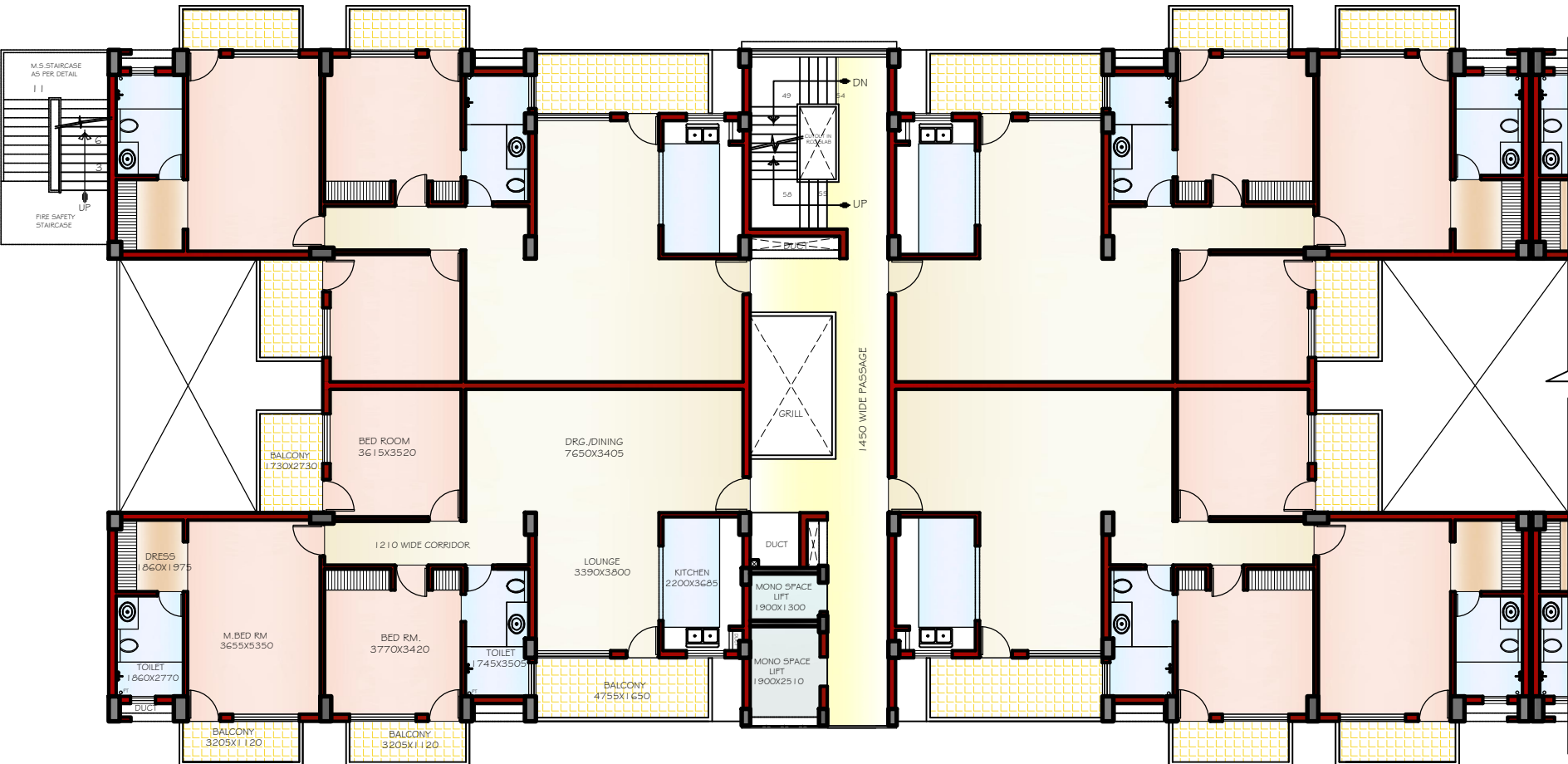
TENTATIVE TYPICAL FLOOR PLAN- 3BHK COVERED AREA - 147 sq.mt.(approx.) ( ALL DIMENSION ARE IN MM.)
