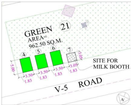
DETAIL - B' 3 NO. PORTA CABIN (3.50MX5.00M EACH) + MILK BOOTH (3.05MX3.05M)
