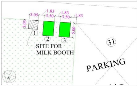
DETAIL - A' 2 NO. PORTA CABIN (3.50MX5.00M EACH) + MILK BOOTH (3.05MX3.05M)
